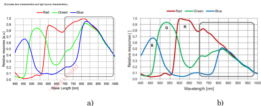
Fig. 6.1. a. Curba QE caracteristica senzorului ASI462MC (color) ( https://astronomy-imaging-camera.com/wp-content/uploads/ASI462-QE-curve.png )
