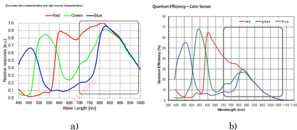
Fig. 2.1. a. Curba QE caracteristica senzorului ASI462MC (color) ( https://astronomy-imaging-camera.com/wp-content/uploads/ASI462-QE-curve.png )
