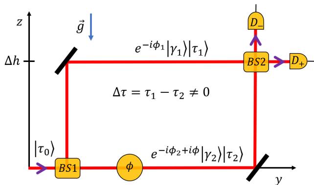
FIG. 3: This figure illustrates the Mach-Zehnder interferometer in Fig. 1 placed in an external gravitational field, i.e. under the influence of a gravitational acceleration \vec{g} . The information about the which-way detector WWD is now encoded in an internal time-evolving degree of freedom that works as a clock. Due to time dilation effects, an initial internal state |\tau_0\rangle can evolve into a linear combination of the two states |\tau_{1,2}\rangle characterized by two different proper times, \Delta\tau = \tau_1 - \tau_2 \neq 0 . The phases \phi_{1,2} depend on the path and on the dynamics of the internal degree of freedom, whereas \phi is a controllable phase shift.
