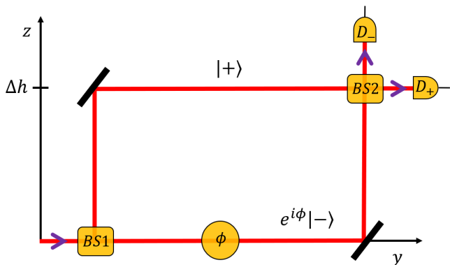
FIG. 1: This figure illustrates a two-way interferometer known as Mach-Zehnder setup. It is made up of two beam splitters BS1, BS2 and two detectors D_{\pm} . The superposed system travels along the two paths that are labeled by |\pm\rangle , and it can generally acquire a relative (controllable) phase shift \phi . The two detectors D_{\pm} measure the degree of interference which appears on the screen as an interference pattern.
