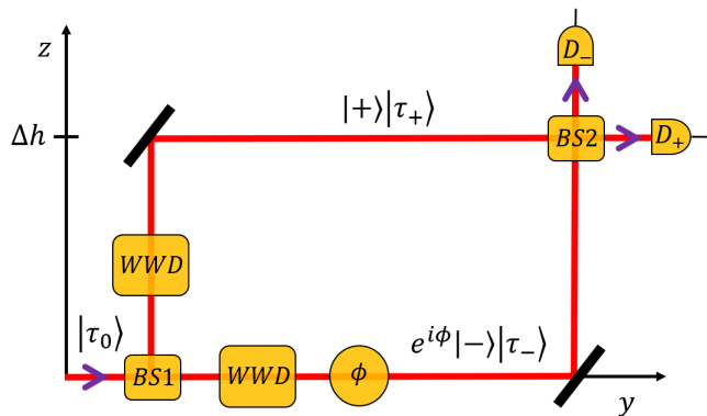
FIG. 2: This figure illustrates the Mach-Zehnder interferometer in Fig. 1 with the addition of an extra degree of freedom that is able to encode the which-way information. Apart from the two beam splitters BS1, BS2 and the two detectors D_{\pm} , we now have a which-way detector indicated by WWD. The main difference with respect to the simpler configuration of Fig. 1 lies in the possibility that the interfering system and WWD can become entangled, thereby allowing to obtain the which-way information from WWD. At the same time, the interferometric visibility \mathcal{V} is reduced, which tells us that the complementarity principle still holds even for a composite system.
