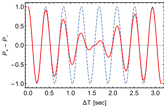
FIG. 4: Quantum interference in GR. The blue dashed line corresponds to the coherent oscillation due to the COW effect, whereas the red solid line represents the interference pattern in the presence of time dilation. One can explicitly notice that, because of time dilation, there is a loss of coherence. For the sake of argument, we have set \Phi' \Delta h \Delta E / (2\hbar c^2) = 1 Hz, m\Phi' \Delta h / \hbar = 15 Hz, \phi = \beta = 0 .
